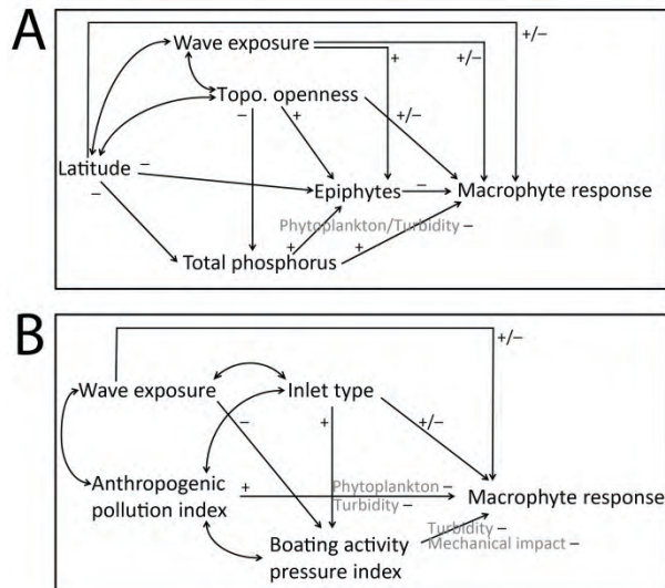
Figure 8. Initial structural models used as starting points in the two analyses ( A and B ), which are explained in the text. Direct paths are indicated by single-headed straight arrows showing direction, while correlations are shown with double-headed curved arrows. Plus (+) or minus (-) signs denote hypothesised positive or negative relationships. Direct relationships with the macrophyte response have both signs (+/-) as the relationship can differ depending on the response studied (cover, number of species, or macrophyte indices). Texts in grey font are variables in a conceptual model. These were not included in the analyses due to lack of data.
